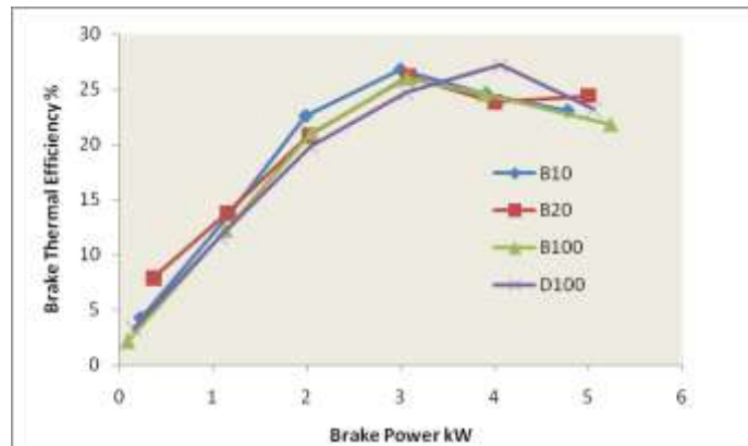
Fig -4: Variation of brake thermal efficiency with brake power
