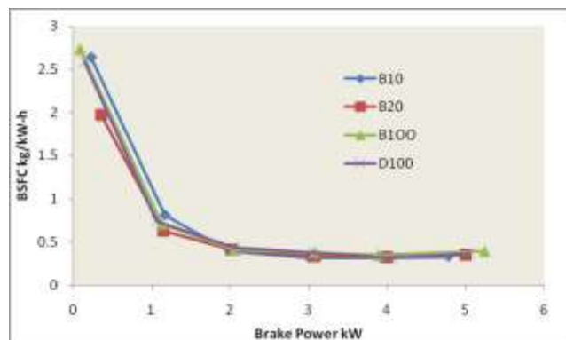
Fig -5: Variation of specific fuel consumption with brake power
