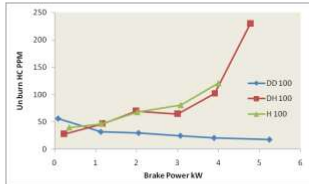
Fig -08: Variation of hydrocarbon with brake power
