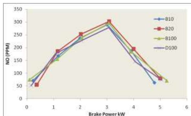
Fig -07: Variation of NOx with brake power
