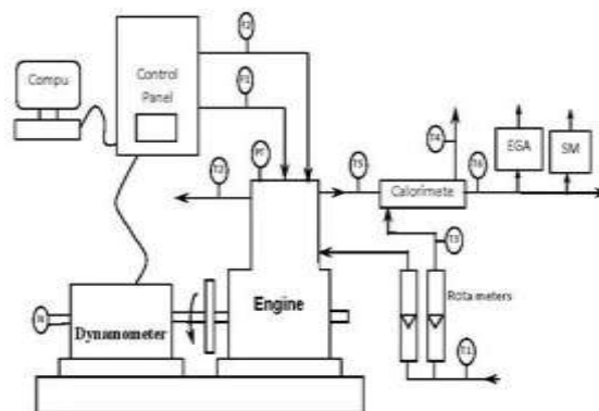
Fig. 2 Experimental Setup
