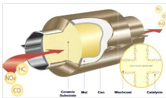
Fig.1. Cut Section of the Catalytic Converter
