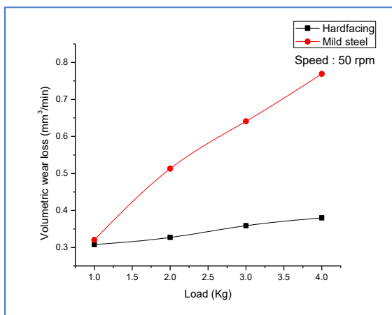
Fig.4 Load-volumetric wear loss
